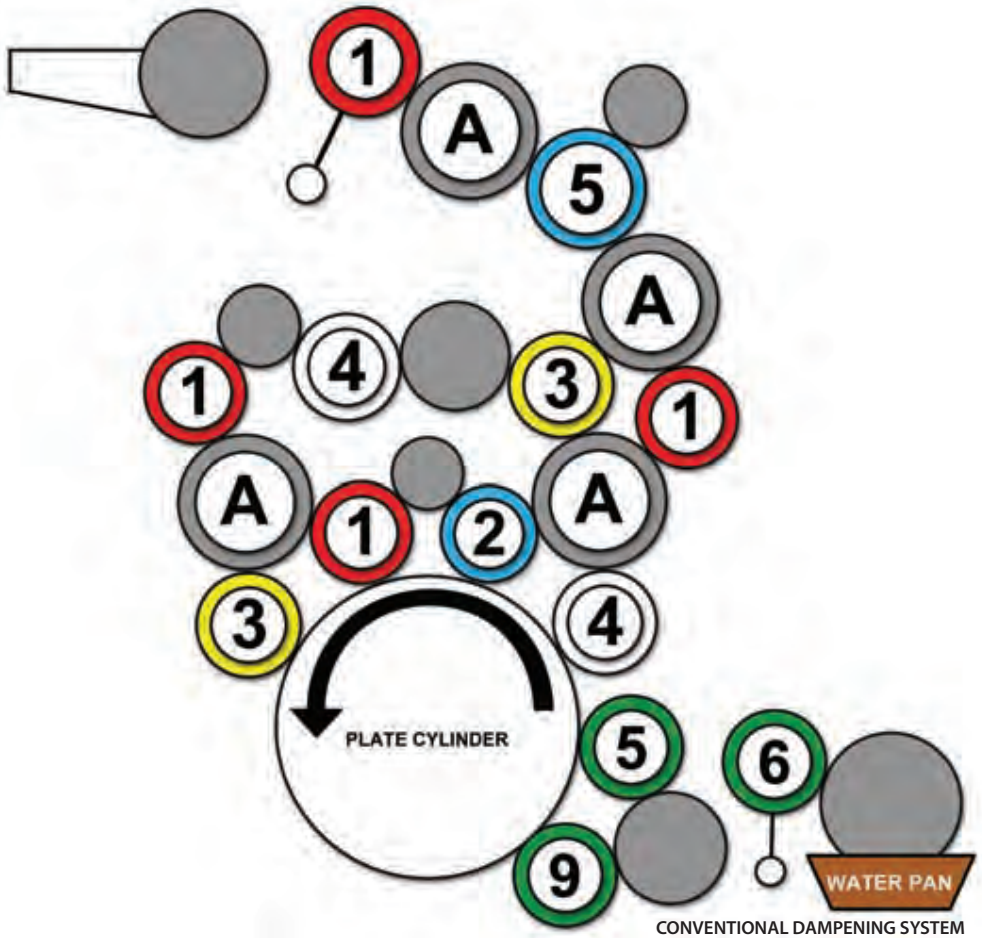
CONVENTIONAL DAMPENING SYSTEM
